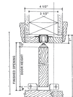
Series 1200 Track Pocket Door Detail Split Header Installation
