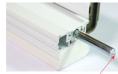
Slide bolt w/machined center punch allows for precise bolt location and ease of installation.
