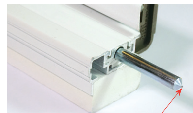
Slide bolt w/machined center punch allows for precise bolt location and ease of installation.
