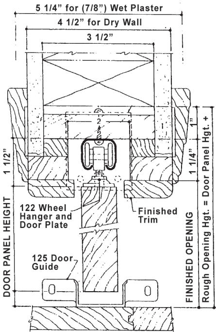
Series 800 Track Pocket Door Detail Under Header Installation
