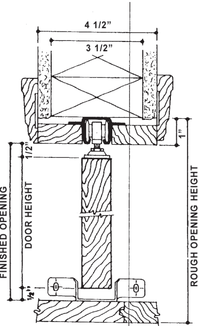
Series 1200 Track Pocket Door Detail Split Header Installation
