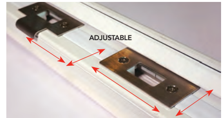
4-way adjustable (horizontal and vertical) strike latch plates
