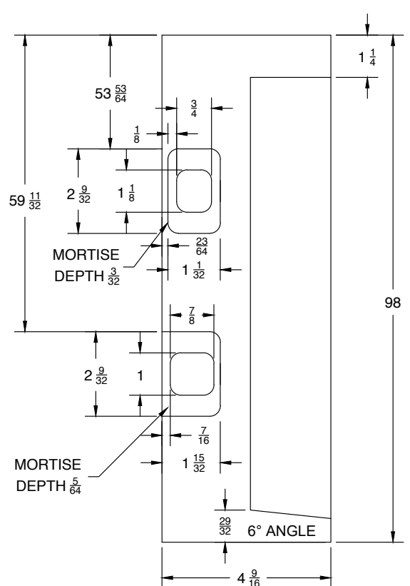
STRIKE JAMB 8/0
