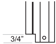
OUTSWING SILL NOTCH
